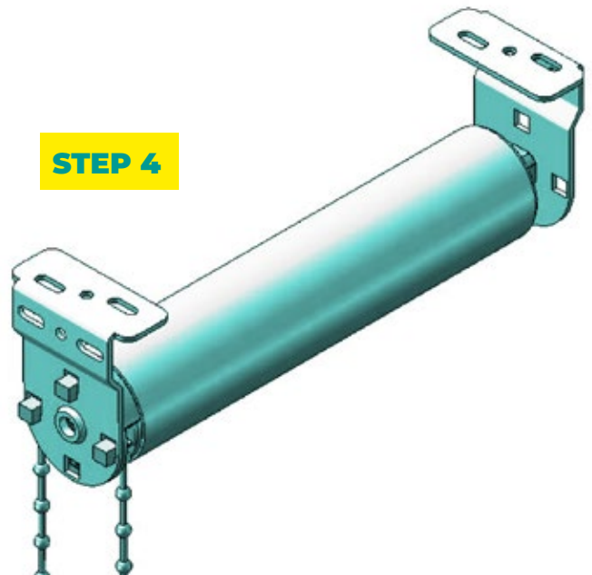
Top fixing
